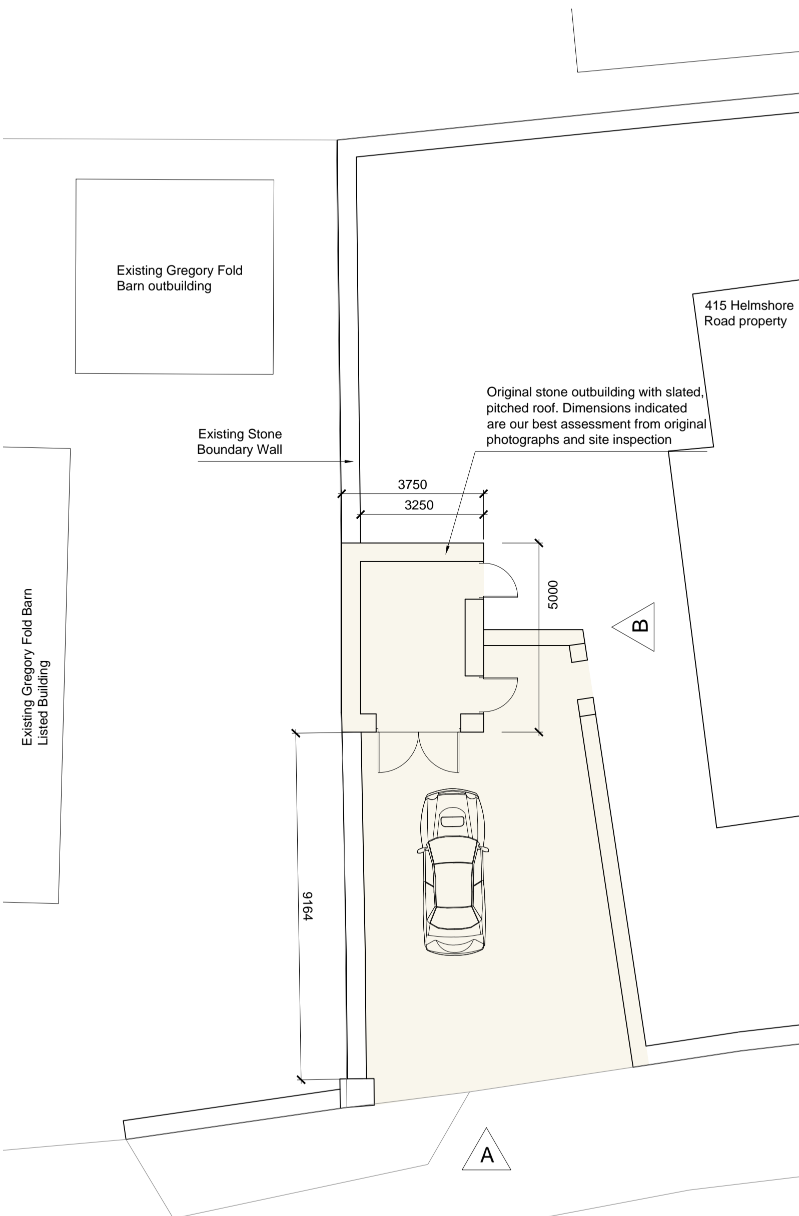
Pre-Existing Plan Detail. Scale 1:100 Pre-Existing Volume = 49 m 3
