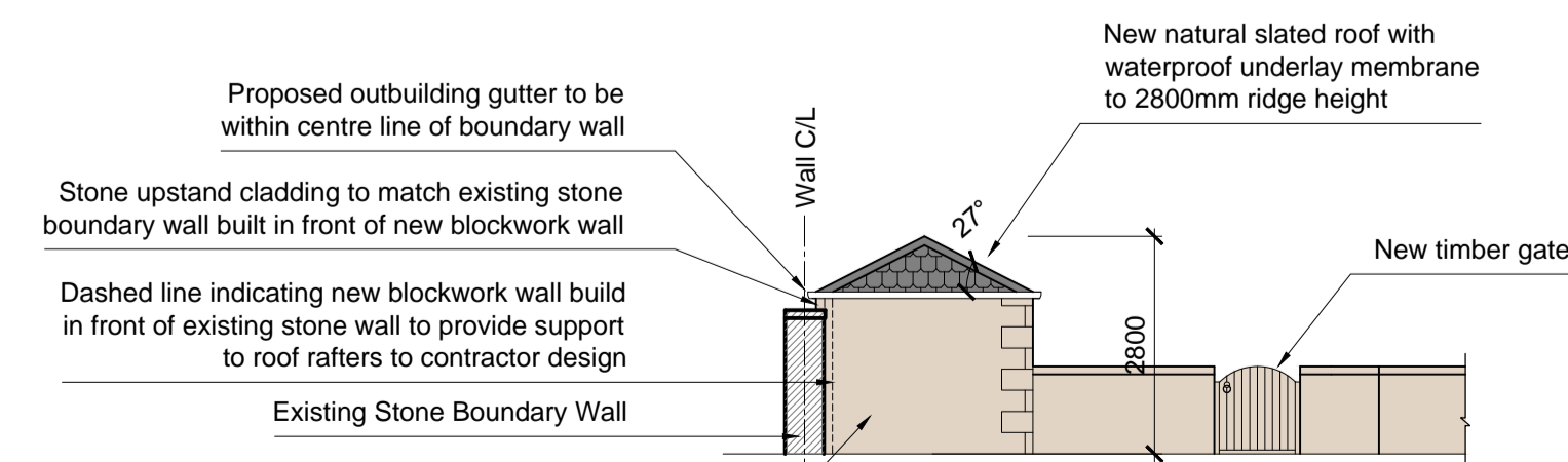
Proposed Elevation A-A Scale 1:100
