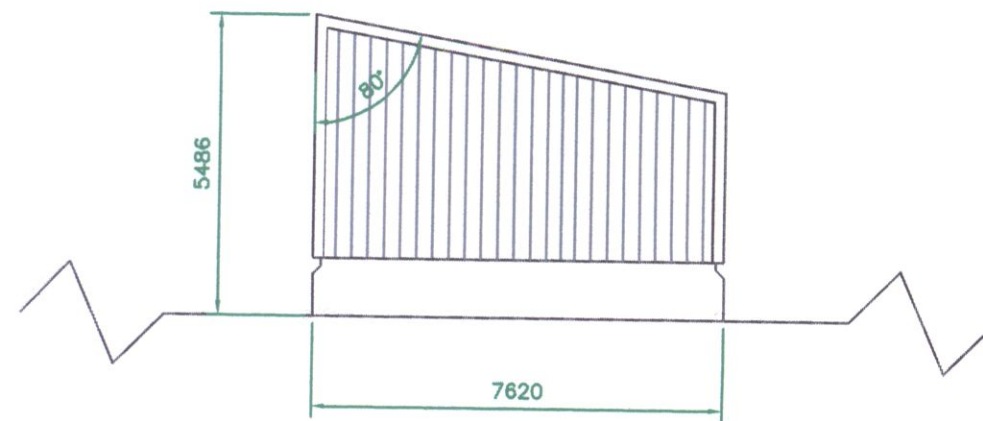
proposed south facing elevation
