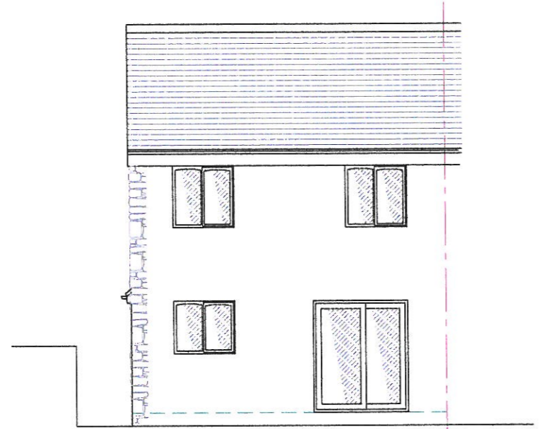
REAR ELEVATION
