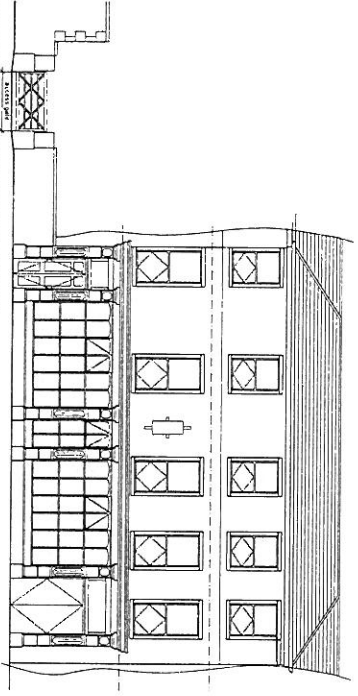
Existing Part Elevation To Manchester Road
