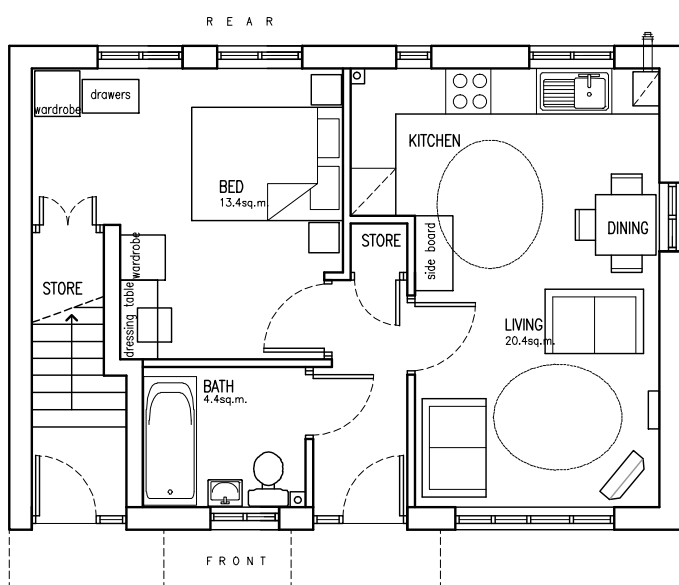
GROUND FLOOR 44sq.m.
