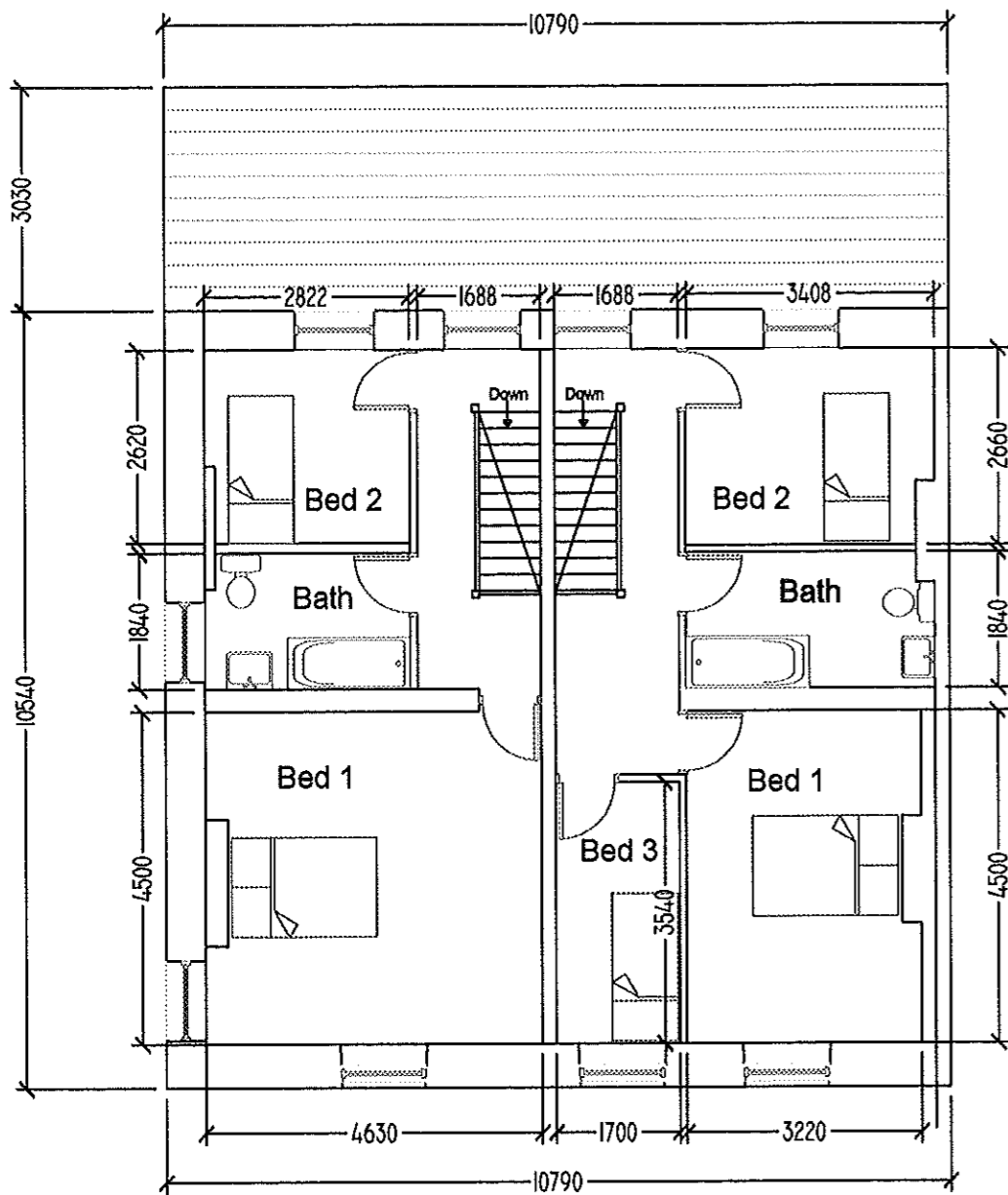
Proposed First Floor Plan 1
