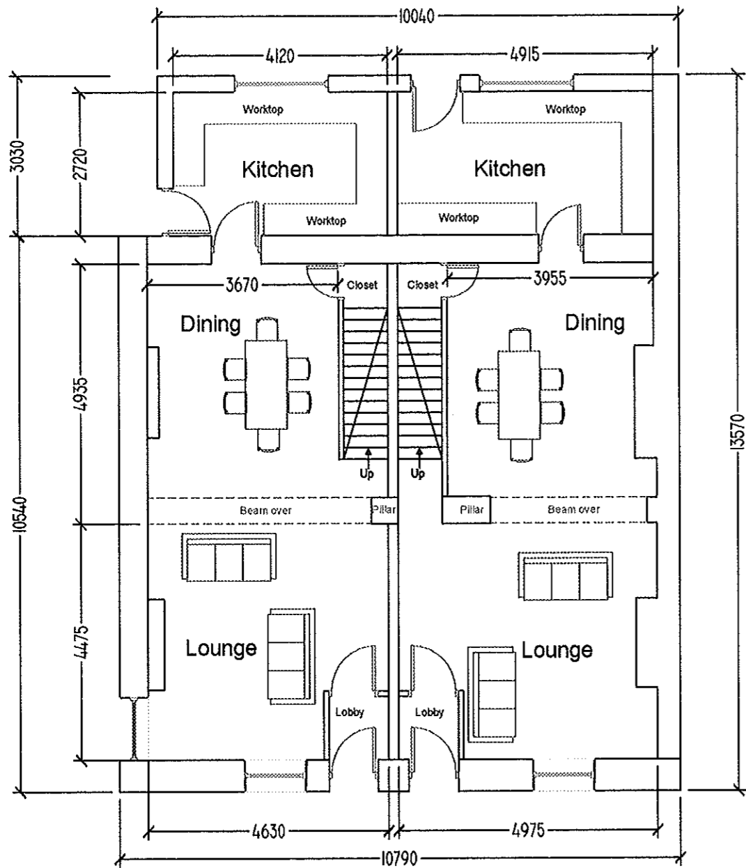
Proposed Ground Floor Plan 2
