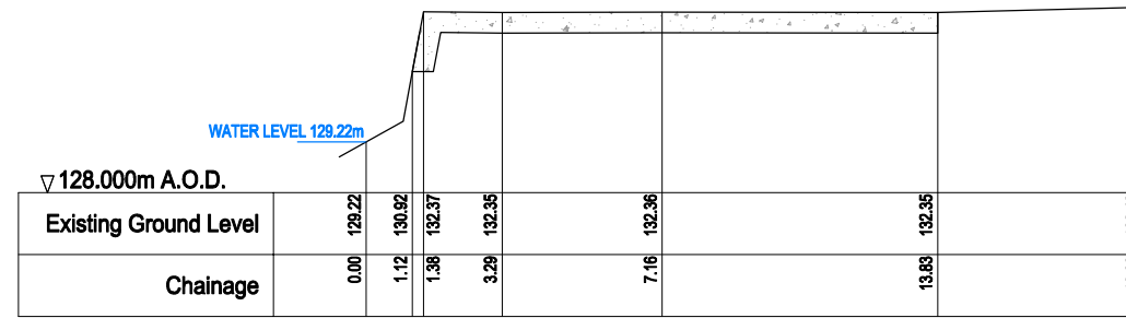
SECTION A-A SECTION THROUGH INLET WEIR SCALE 1:100 A1, 1:200 @ A3
