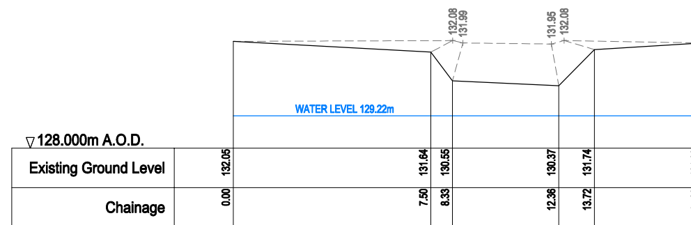
SECTION D-D SECTION ACROSS OUTLET WEIR SCALE 1:100 A1, 1:200 @ A3
