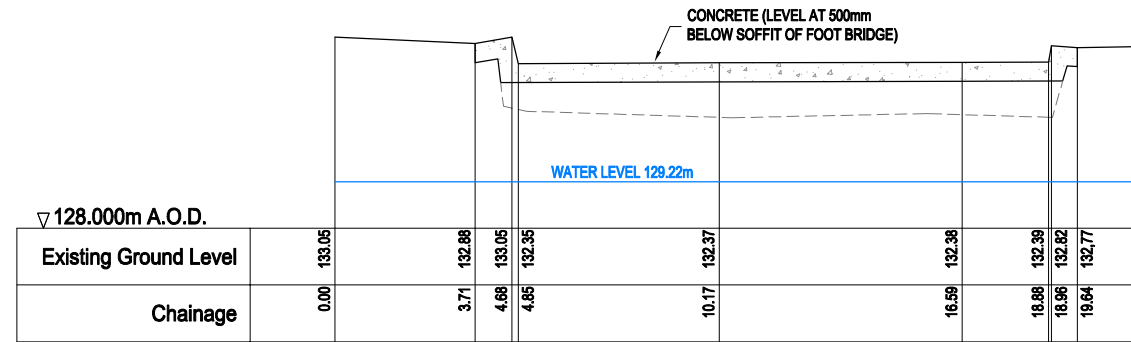
SECTION B-B SECTION ACROSS INLET WEIR SCALE 1:100 A1, 1:200 @ A3
