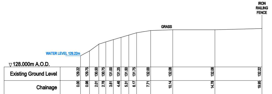
SECTION C-C SECTION THROUGH OUTLET WEIR SCALE 1:100 A1, 1:200 @ A3
