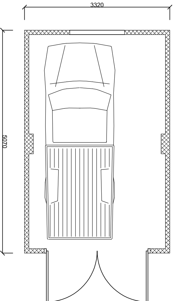
PLAN
