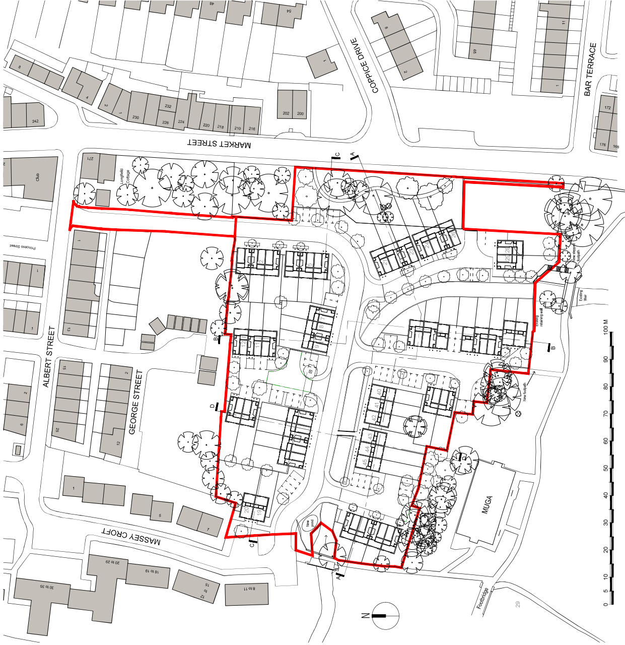
PROPOSED SITE LAYOUT 1 : 500 scale
